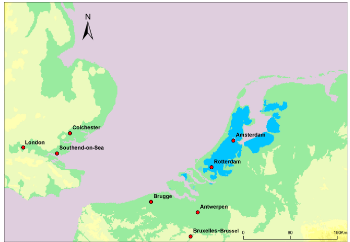
Figure 7: Areas flooded (in blue) by sea level rise for three different sea levels, assuming the absence of dykes 9
